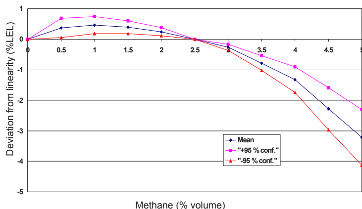
Figure 2 Linearity
