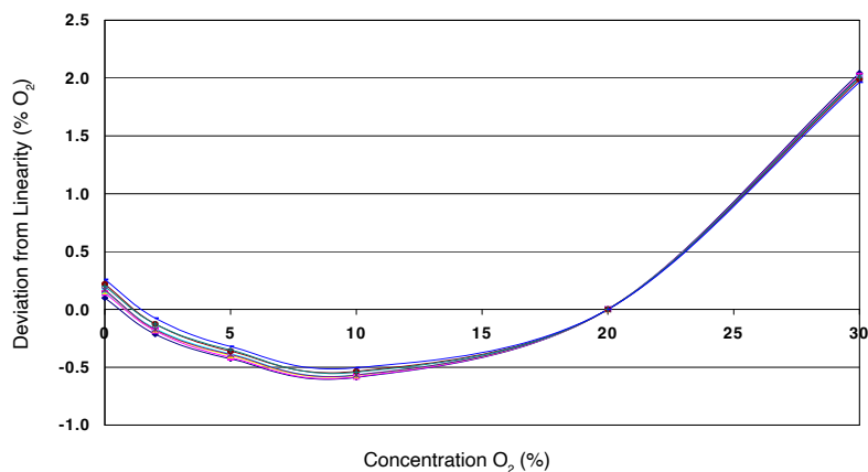
Figure 3 Linearity
