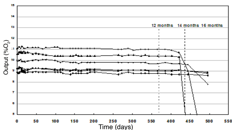
Figure 3 Long-Term Stability
