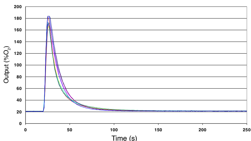
Figure 2 Pressure Step Performance
