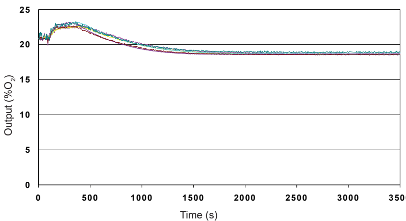
Figure 3 Thermal Transient Performance
