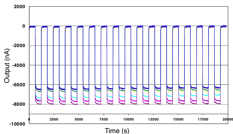
Figure 3 Repeated gassing with 20ppm NO 2
