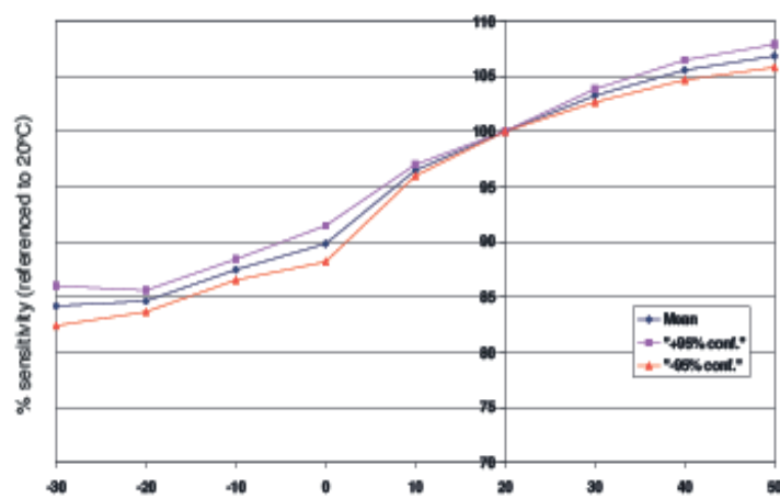
Figure 1 Sensitivity Temperature Dependence
