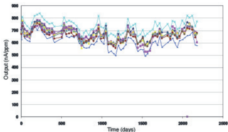
Figure 3 Sensitivity Long-term Stability
